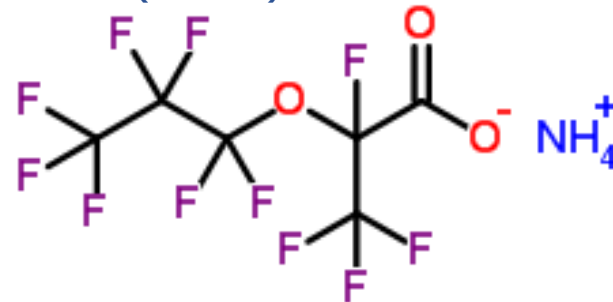
FRD-903 (GenX)
